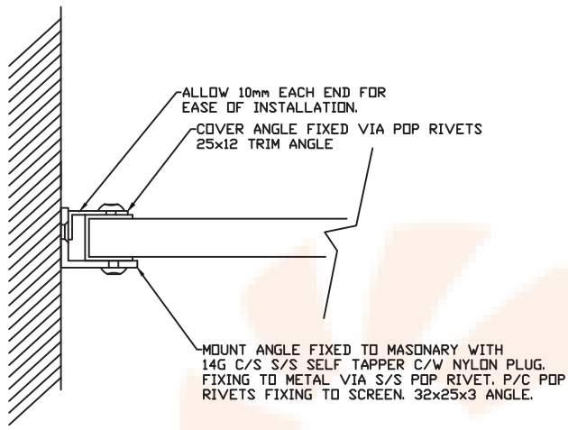
FIXING DETAIL
